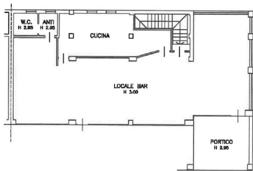
PIANO TERRA
